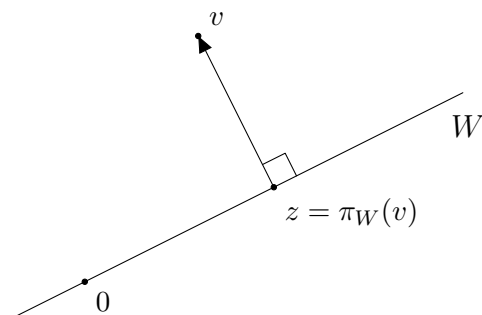
FIGURE 1.12. Orthogonal projection of v onto a line or hyperplane W with 0 \in W
