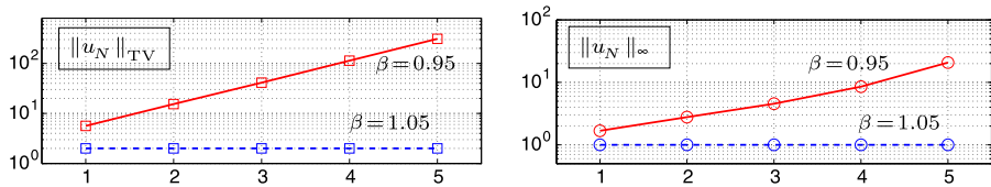
Fig. 3 Values of \|u_N\|_{TV} (left) and \|u_N\|_\infty (right) for T = 1, 2, \dots, 5 and the two-step methods (2.1) with \beta = 1.05 (dashed), \beta = 0.95 (solid lines)
