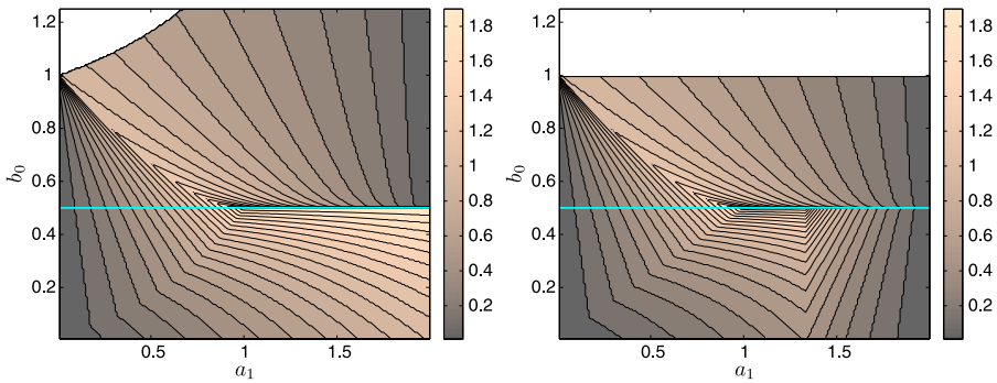
Fig. 5 Implicit two-step methods of order two, with parameters a_1 \in [0, 2) horizontally and b_0 \in [0, \frac{5}{4}] , b_0 \neq \frac{1}{2} , vertically. Left panel: thresholds \gamma > 0 for boundedness. Right panel: thresholds \gamma > 0 for monotonicity with the \theta -method, \theta = b_0 , as starting procedure. Contour levels at j/10 , j = 0, 1, \dots ; for the ‘white’ areas there is no positive \gamma
