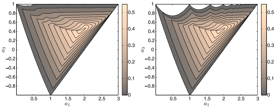
Fig. 6 Explicit three-step methods of order three, with parameters a_1 \in [0, 3] horizontally and a_3 \in [-1, 1] vertically. Left panel: threshold \gamma > 0 for boundedness, that is, P \geq 0 and -\gamma \in \text{int}(S) . Right panel: maximal \gamma > 0 such that P \geq 0 and R \geq 0 . Contour levels at j/20, j = 0, 1, \dots ; for the ‘white’ areas there is no positive \gamma
