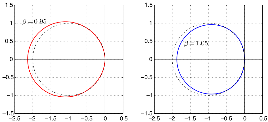
Fig. 1 Stability regions of the two-step methods (2.1) with \beta = 0.95 (left), \beta = 1.05 (right). For comparison, the circle \{\zeta \in \mathbb{C} : |\zeta + 1| = 1\} is displayed by the dashed curve
