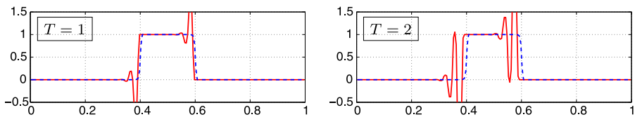
Fig. 2 Numerical solutions at T = 1 and T = 2 for the two-step methods (2.1) with \beta = 1.05 (dashed), \beta = 0.95 (solid lines)
