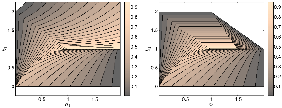
Fig. 4 Explicit two-step methods of order one, with parameters a_1 \in [0, 2) horizontally and b_1 \in [-\frac{1}{4}, \frac{9}{4}] , b_1 \neq 1 , vertically. Left panel: threshold \gamma > 0 for boundedness. Right panel: threshold \gamma > 0 for monotonicity with forward Euler starting procedure. Contour levels at j/20 , j = 0, 1, \dots ; for the ‘white’ areas there is no positive \gamma
