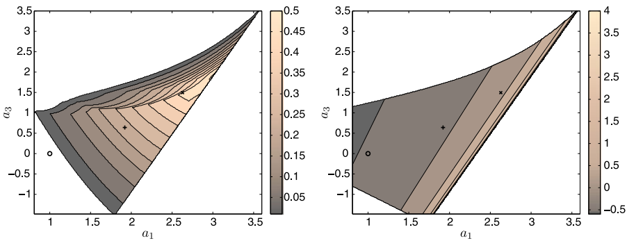
Fig. 7 Explicit four-step methods of order four, with parameters described in the text. Left panel: threshold \gamma > 0 for boundedness. Contour levels at j/20, j = 0, 1, \dots ; for the ‘white’ areas there is no positive \gamma . Right panel: \log_{10} of the absolute error constants for zero-stable methods. Markers: \circ for AB4, + for EBD4 and \times for TVB(4,4)
